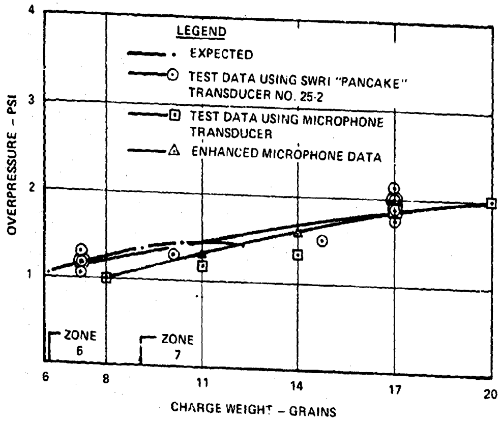
Figure 11. Comparison of Predicted and Model Overpressure Measurements at 40 Calibers Off Boresight
