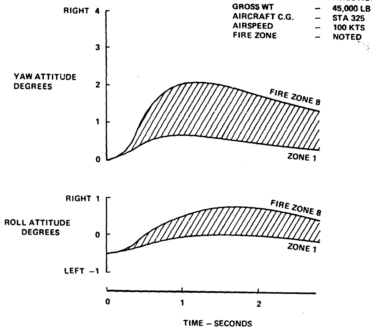
Figure 31. Responses to Recoil Increase With Increased Firing Zone
