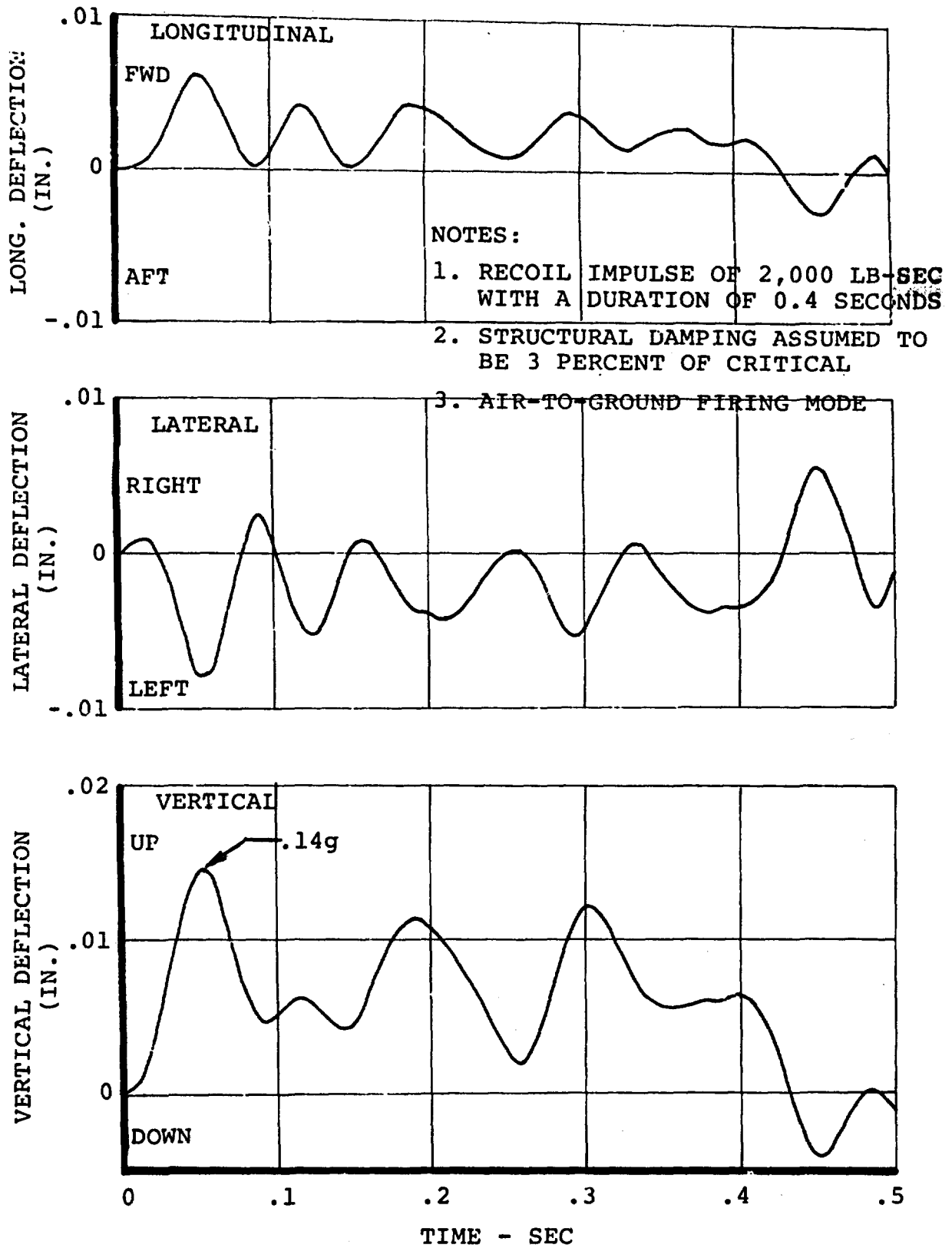
Figure 35. Deflection Response of the Cockpit Due to the Recoil Load from a Single Firing of One Weapon
