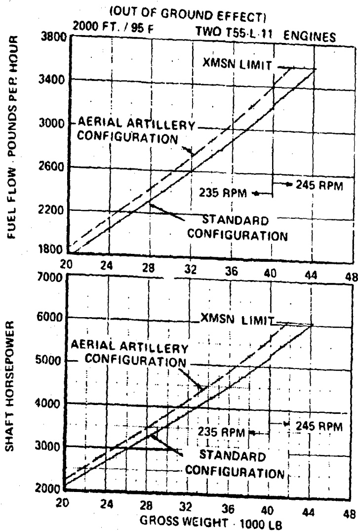
Figure 46. CH-47C Helicopter Hover Power and Fuel Flow Versus Gross Weight
